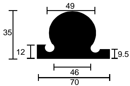
F 637 EPR 55 N
