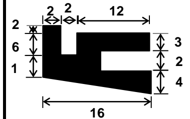
F 480 CR50G
